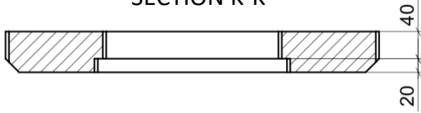
SECTION K-K
